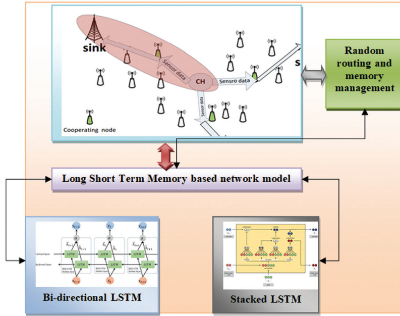
Figure 2: Generic view of the proposed model
