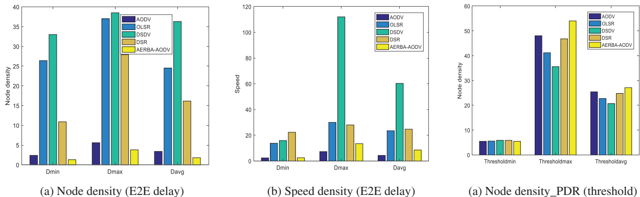
Figure 3: (a) Node density (E2E delay) (b) Speed density (E2E delay) (a) Node density_PDR (threshold)
