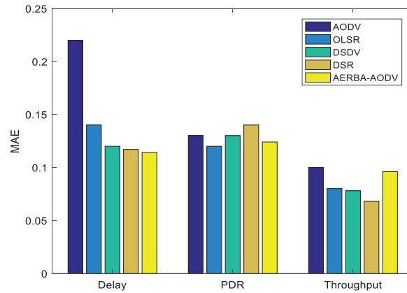
Figure 6: MAE computation
