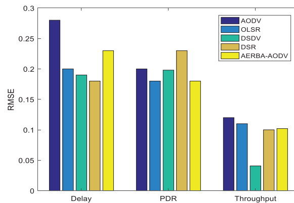
Figure 5: RMSE computation
