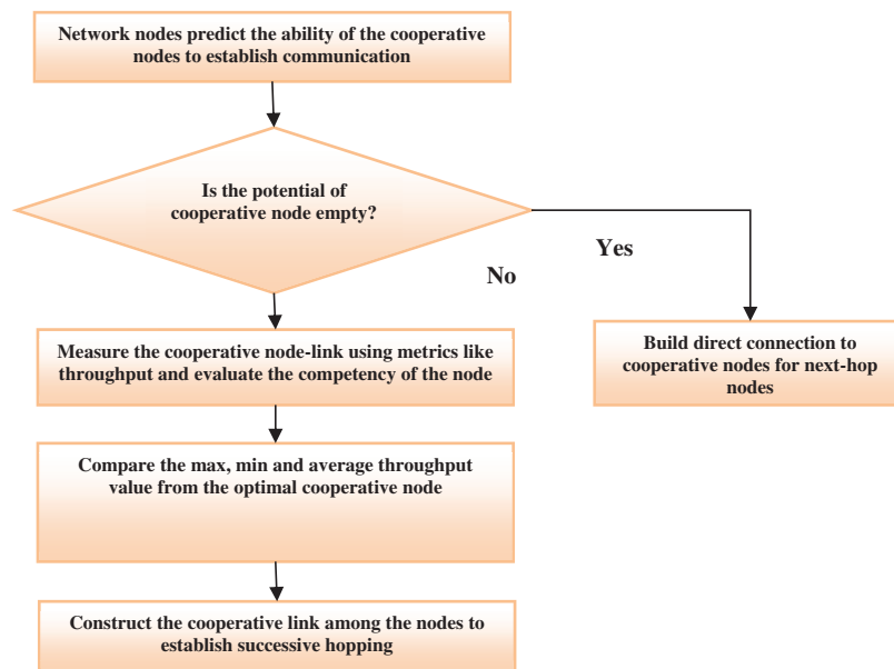
Figure 1: Cooperative node selection process
