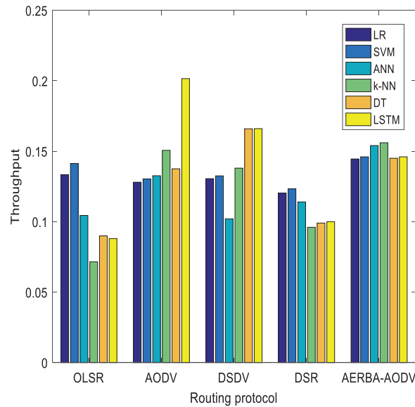
Figure 7: Throughput comparison of proposed vs. existing approaches
