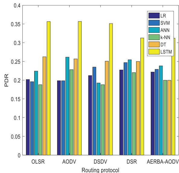
Figure 9: PDR comparison of proposed vs. existing approaches
