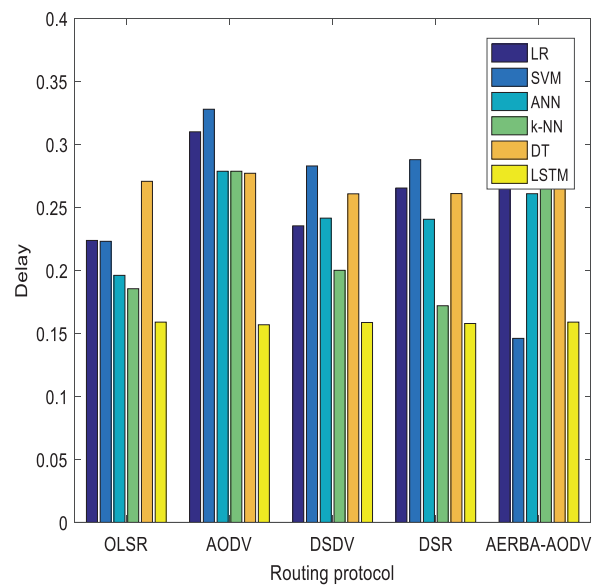
Figure 8: E2E delay comparison of proposed vs. existing
